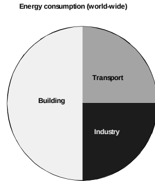
Figure 2 World-wide energy consumption distribution (Behling et al. 1996)
