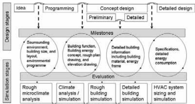
Figure 5 Linking design and simulation in the conceptual design stage (modified from Xia et al.)
