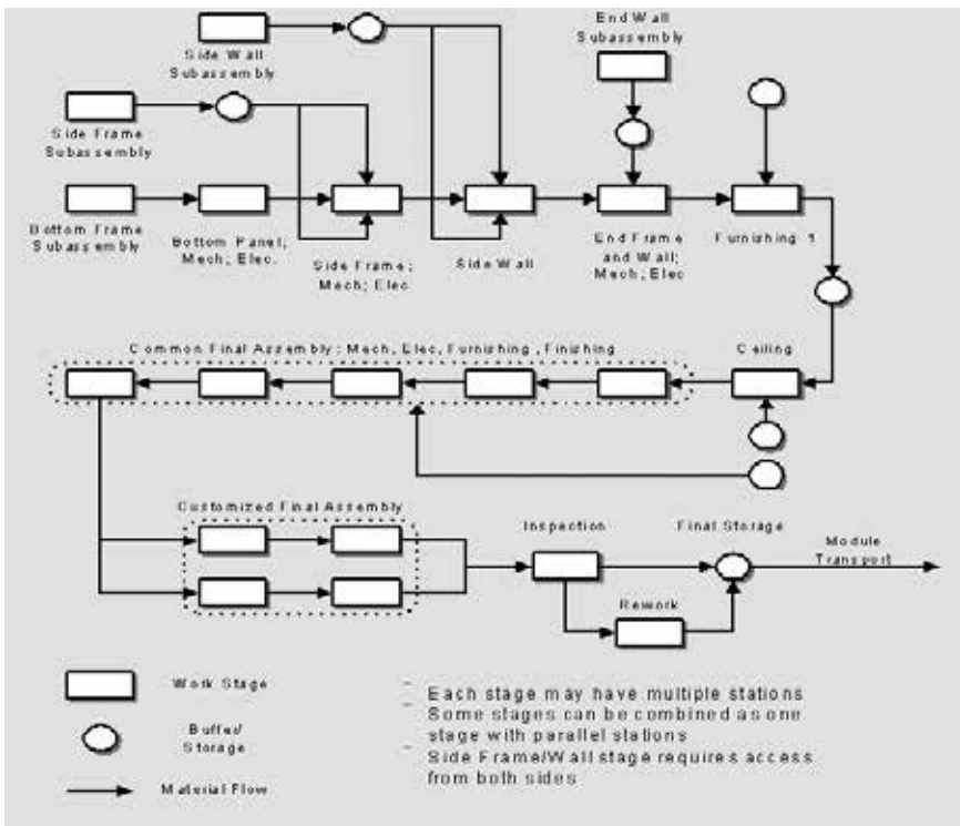
Figure 19 A model for a customized modular housing production line
