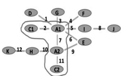
Assembly Sequence I
